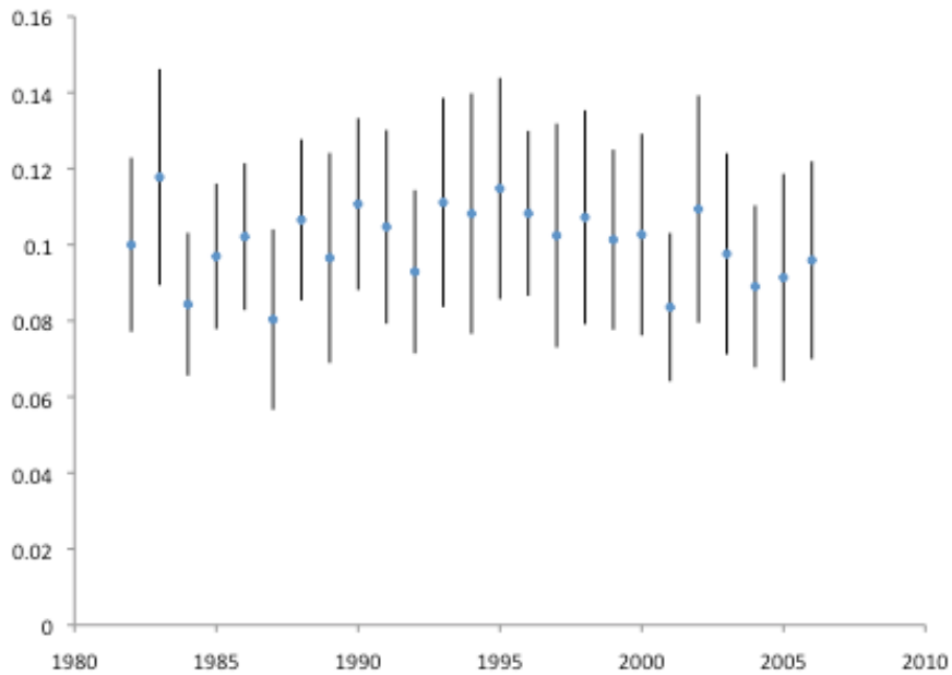
Figure A2.3: Mean spring NDVI for the Uzbek Ustyurt, 1981 – 2006 from the GIMMS data set. Error bars show the standard deviation
